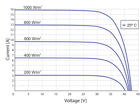
I-V Curve at Various Irradiation Levels
