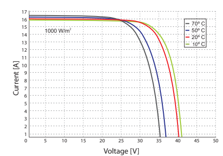
I-V Curve at Various Cell Temperatures
